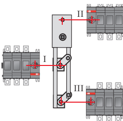
Bypass switches
