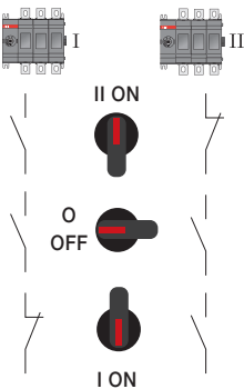
Change-over switches
