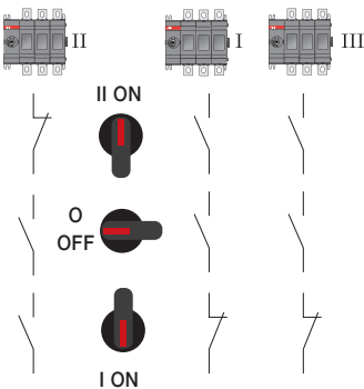
Bypass switches
